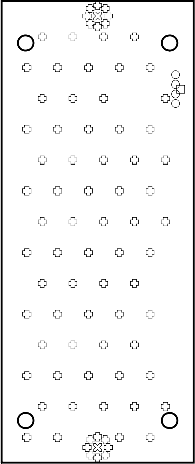
Drill Drawing View (Scale 1:1)
